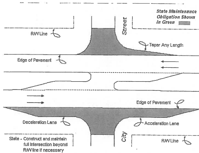
EXISTING CITY STREET CROSSED AT GRADE BY NEW STATE HIGHWAY
