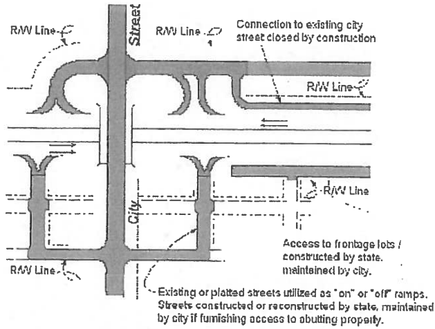
TYPICAL LIMITED ACCESS HIGHWAY UTILIZING CITY STREETS AS "ON" AND "OFF" RAMPS
